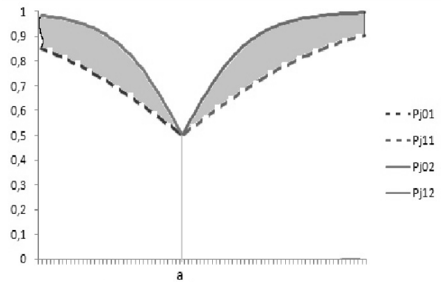
Figure 1.1.b. The item characteristic curve for calculating the uniform DIF index in PCM with 2 categories
