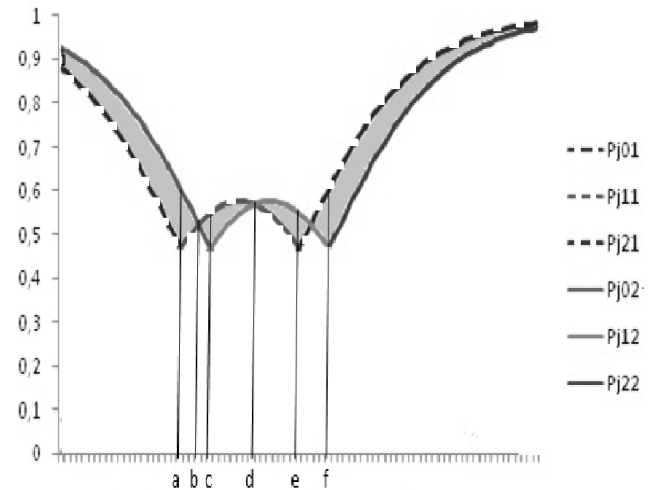
Figure 1.4.b. Part of the CRF that might be used in calculating the integral of non-uniform DIF loads index in 3 categories
