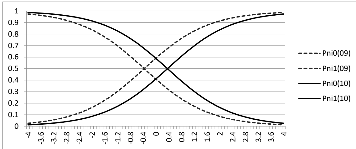
Figure 4.2. the Graphic of Category Response Function for the item CR127
