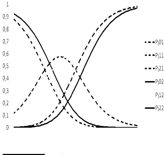
Figure 1.4.a. The CRF with 3 categories (containing non-uniform DIF loads)
