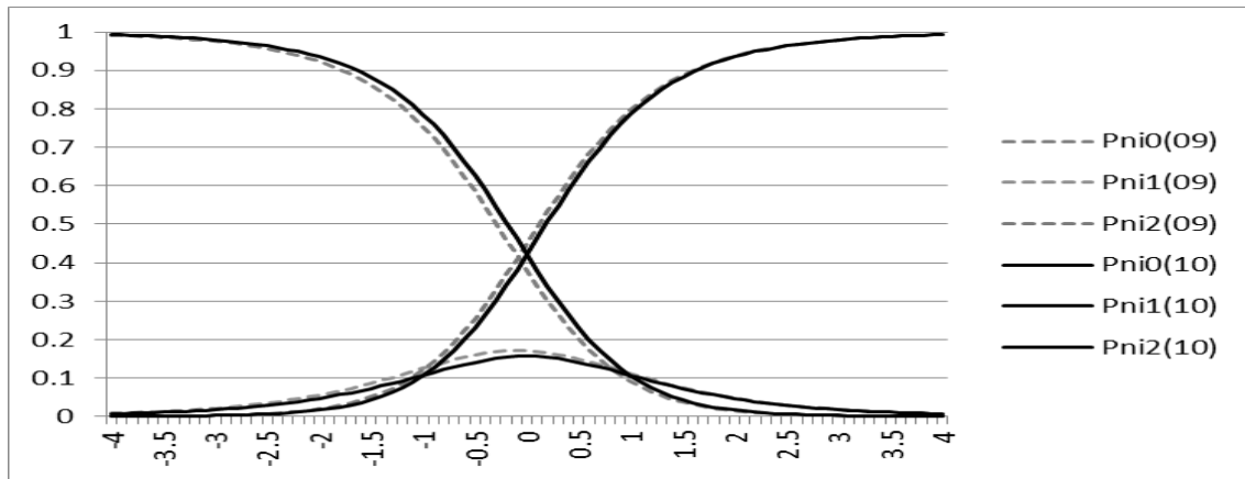
Figure 4.5. The Graphic of Item Response Category for the Item CR225
